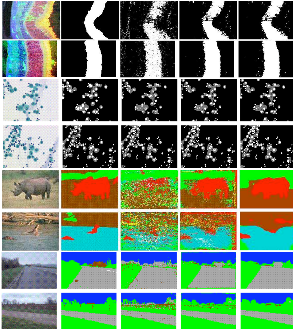
From left to right: original image, manual annotation, annotations by PCM, SCM, and SCMMO. From top to bottom: Retina, Bronchial, Corel, and Sowerby.
