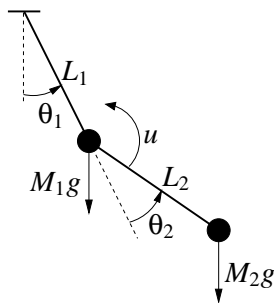
Figure 20: Representation of the Acrobot.
