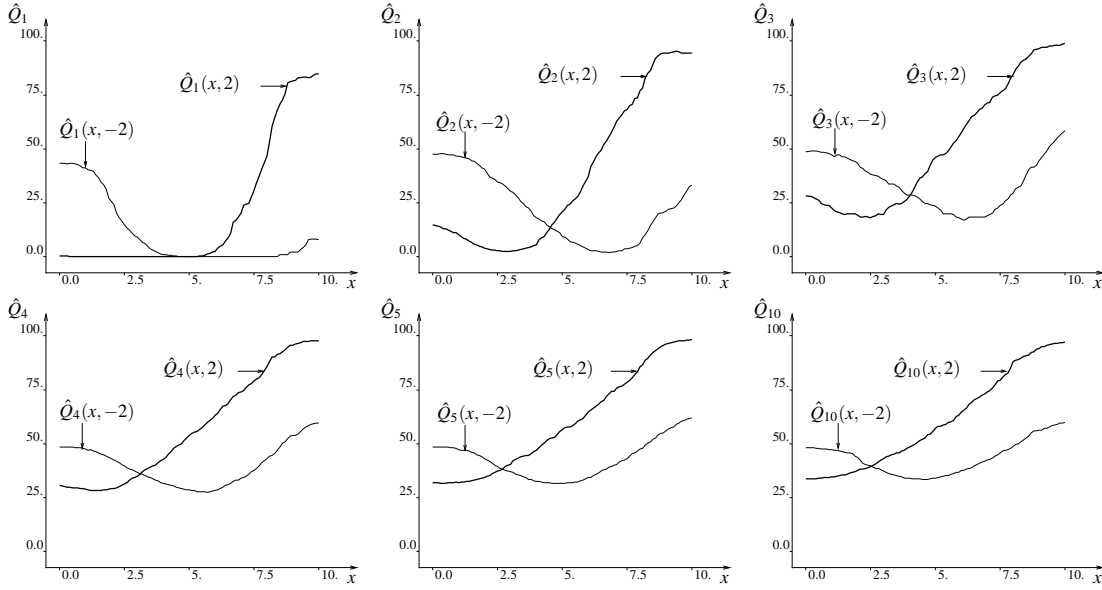
Figure 5: Representation of \hat{Q}_N for different values of N . The set \mathcal{F} is composed of 2010 elements and the supervised learning method used is the Pruned Extra-Trees.
