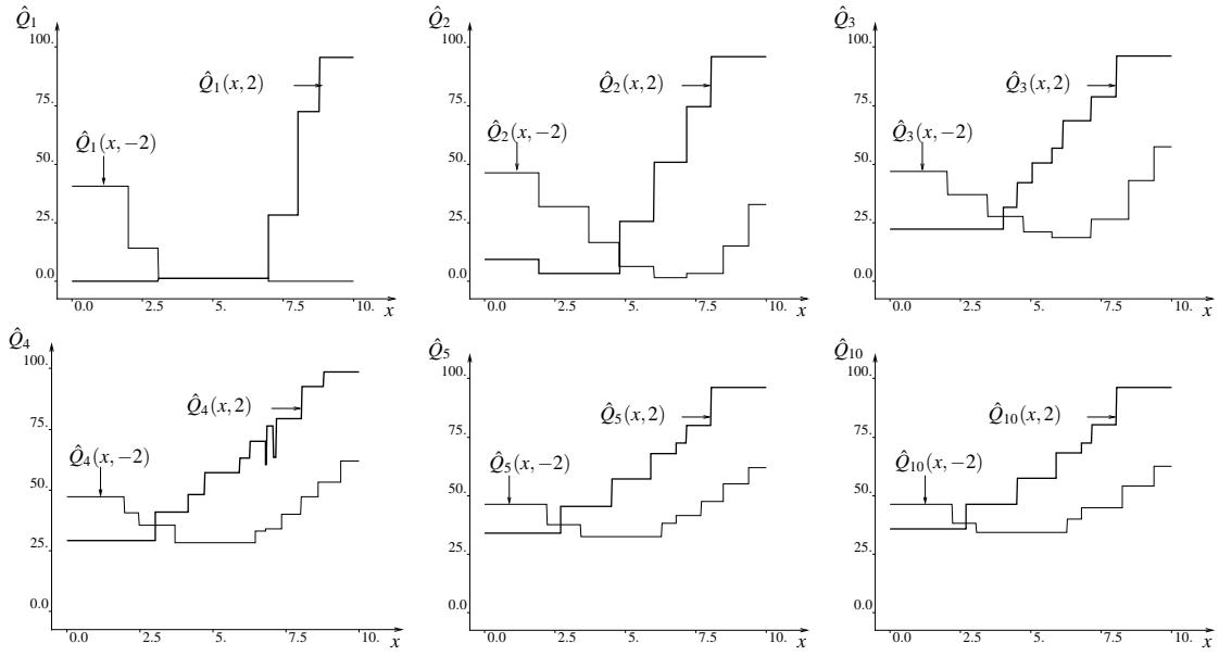
Figure 3: Representation of \hat{Q}_N for different values of N . The set \mathcal{F} is composed of 2010 elements and the supervised learning method used is Pruned CART Tree.
