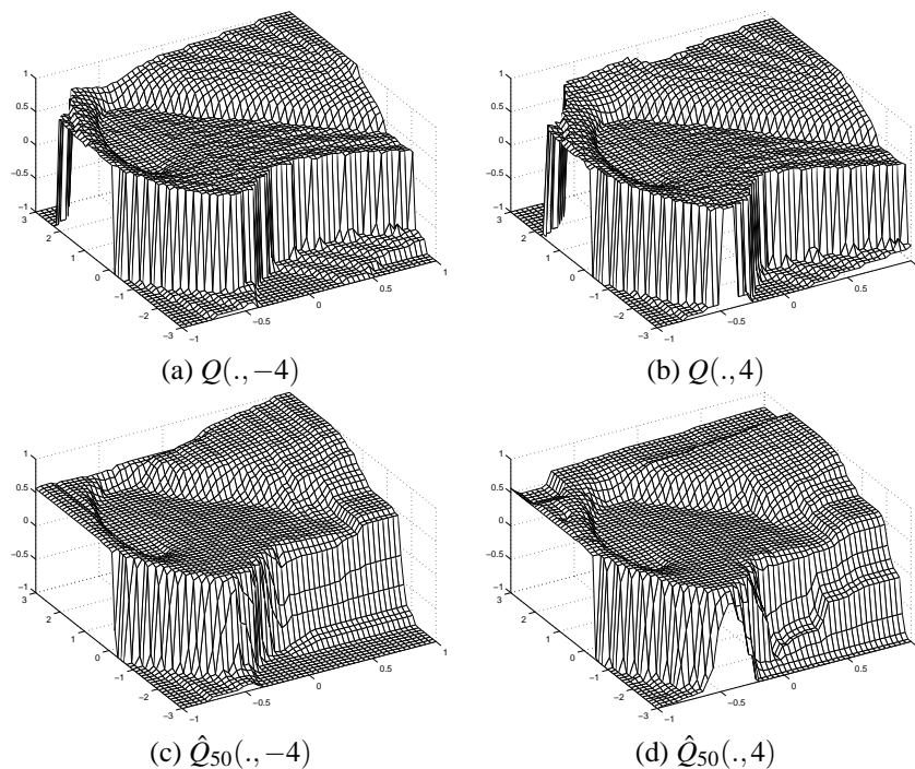
Figure 12: Representation of the Q -function and of \hat{Q}_{50} . \hat{Q}_{50} is computed by using fitted Q iteration together with Tree Bagging.
