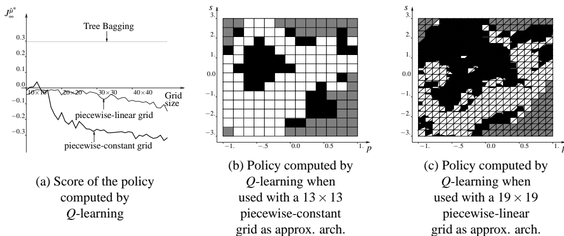
Figure 16: Q -learning with piecewise-constant and piecewise-linear grids as approximation architectures. Each element of \mathcal{F} is used once to refresh the estimate of the Q -function. The set \mathcal{F} is composed of the four-tuples gathered during 1000 episodes.
