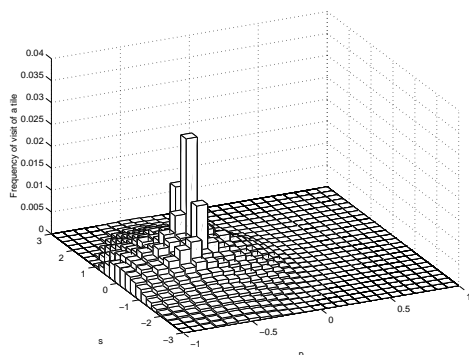
Figure 11: Estimation of the x_t distribution while using episodes starting from (-0.5, 0) and choosing actions at random.
